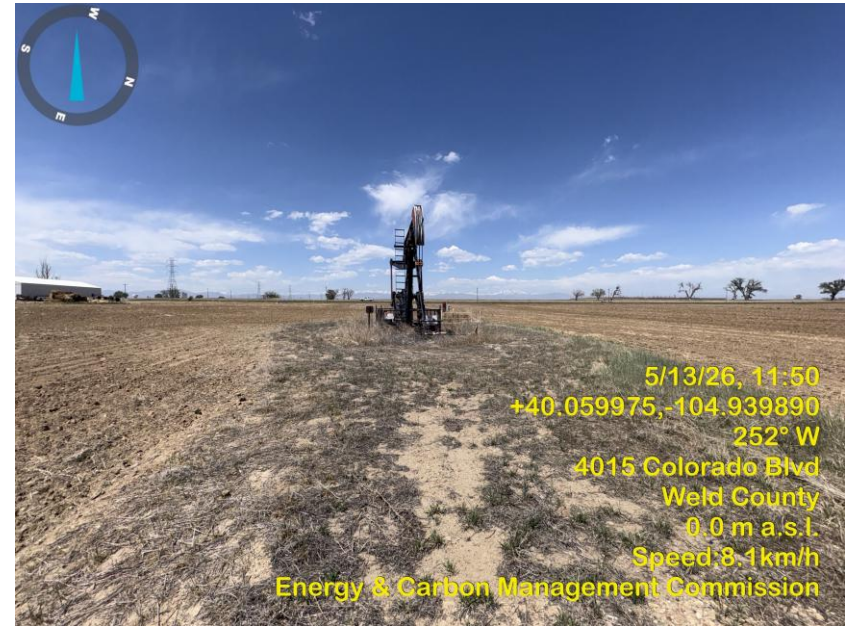
Photo 2 Wellsite.
