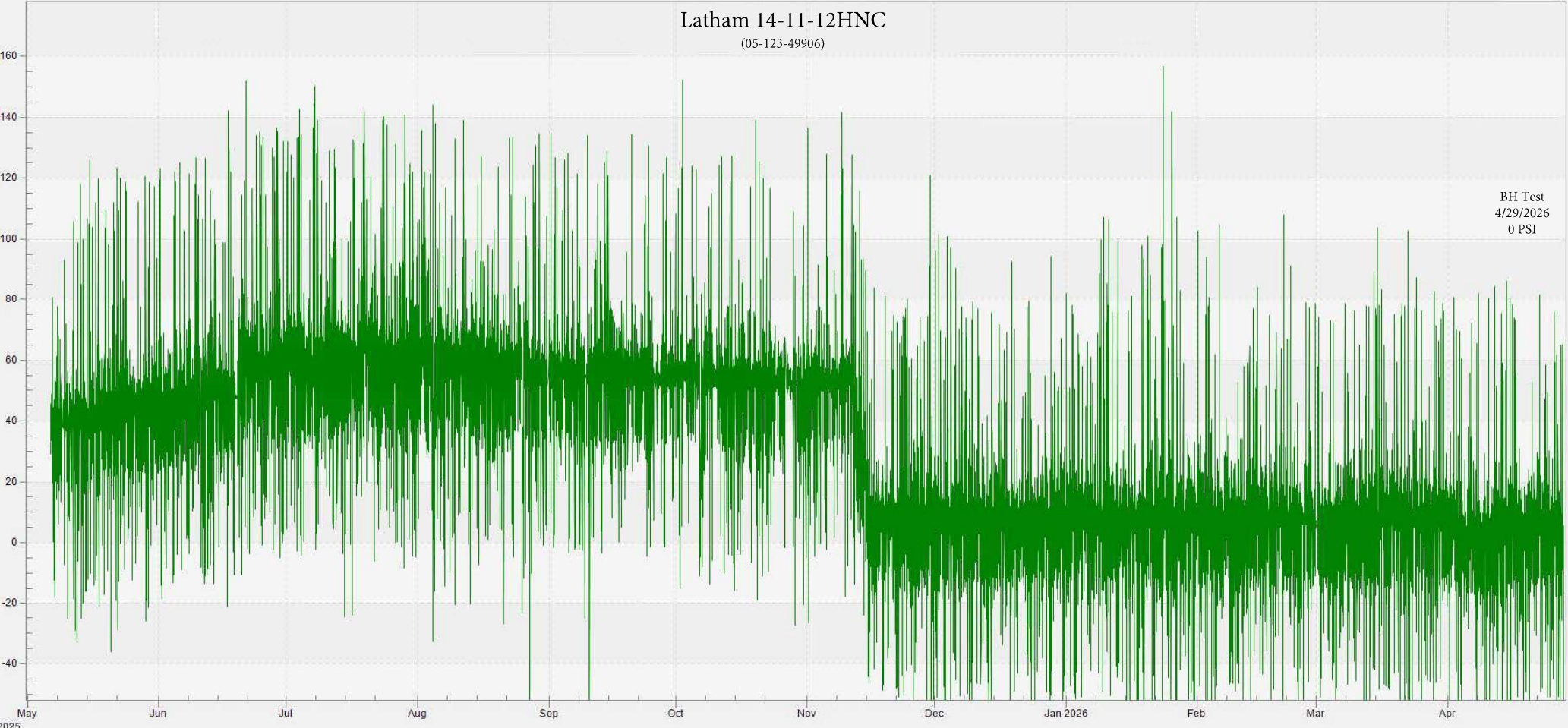
Latham 14-11-12HNC Well Surface Casing Pressure
