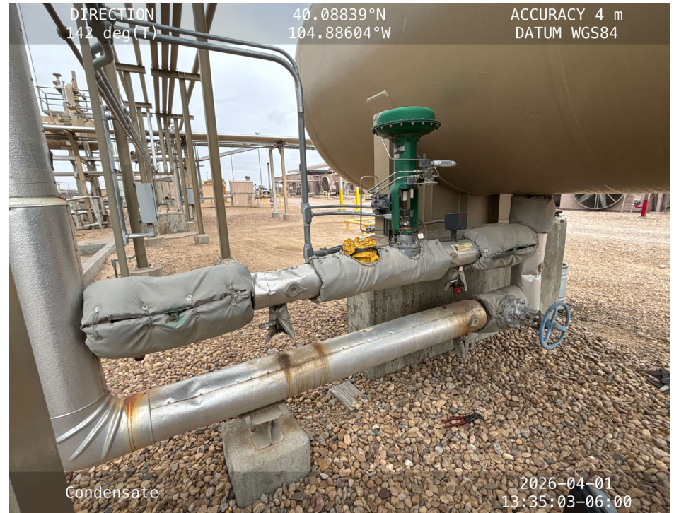
6-inch steel high pressure gas gathering pipeline sample location
