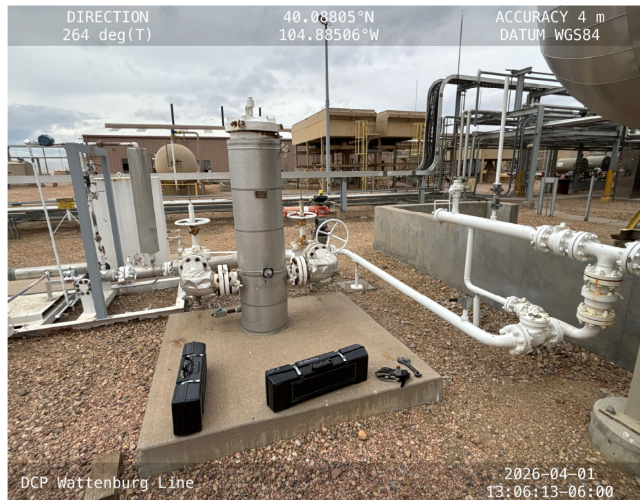
4-inch steel high pressure natural gas liquid (NGL) pipeline (AKA Wattenburg Pipeline) sample location
