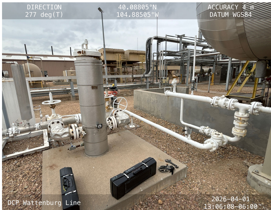
Constant pressure floating piston sample cylinder (CP cylinder) carrying cases
