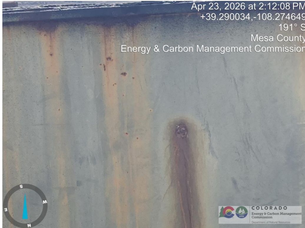
Seep hole on side of tank.
