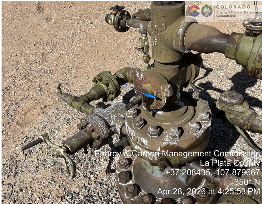
5. Close up of wellhead. Valve handle removed below pen.
