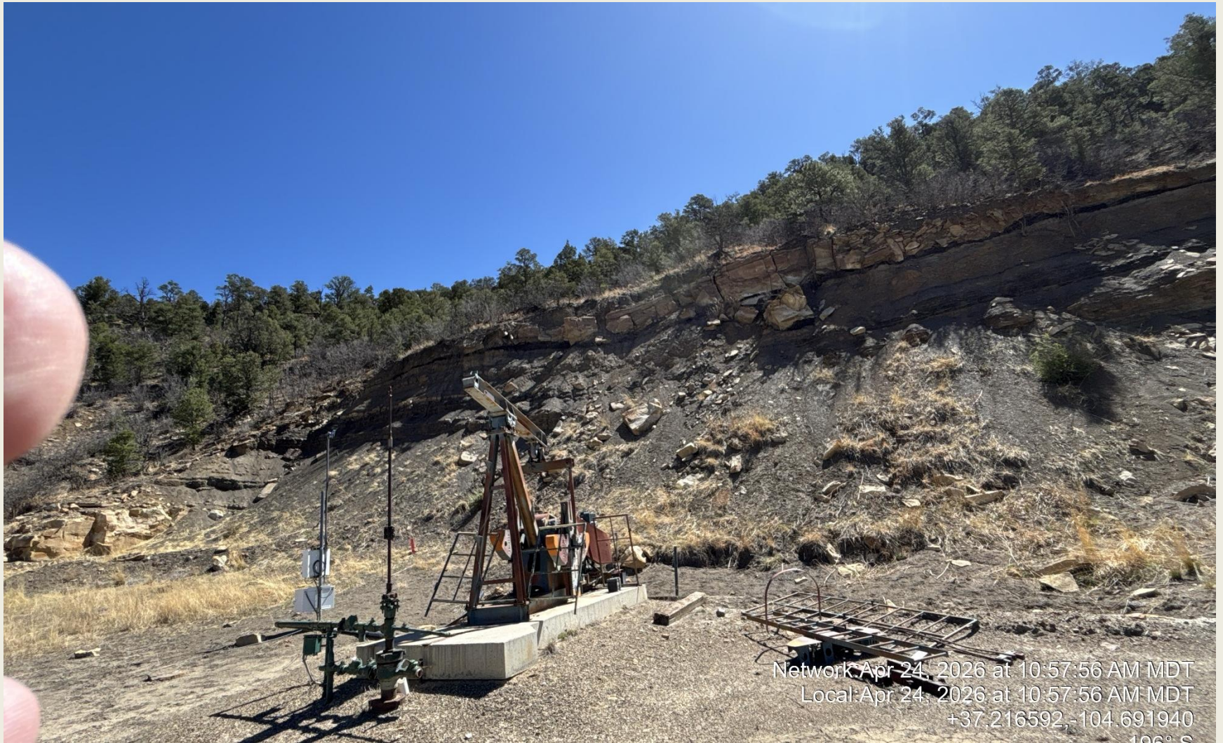
PHOTO 4: WELLHEAD AND EQUIPMENT. UNUSED EQUIPMENT (HEAD FOR PUMPJACK, JUMPJACK FENCING AND WOOD CHOCK ON GROUND NEAR JUMPJACK. REMOVE OR REINSTALL UNUSED EQUIPMENT PER RULE 606. CA DATE 5/24/2026.
