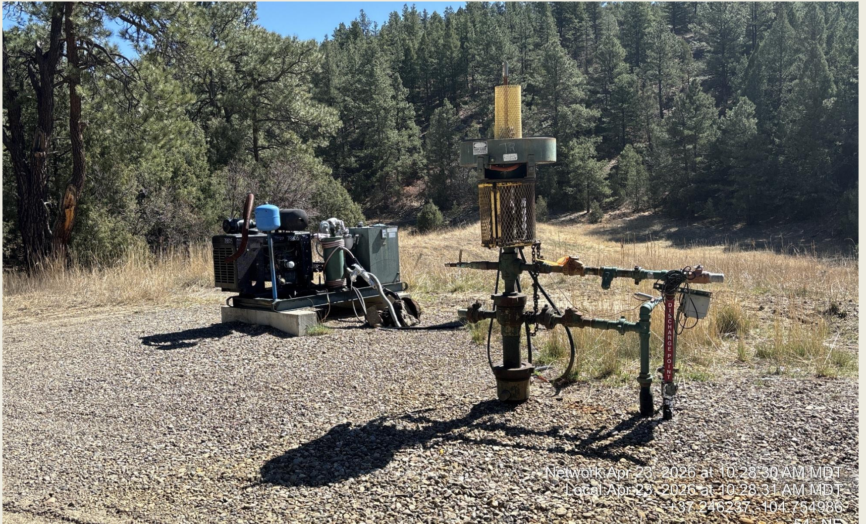
PHOTO 5: TR WELLHEAD AND EQUIPMENT.
