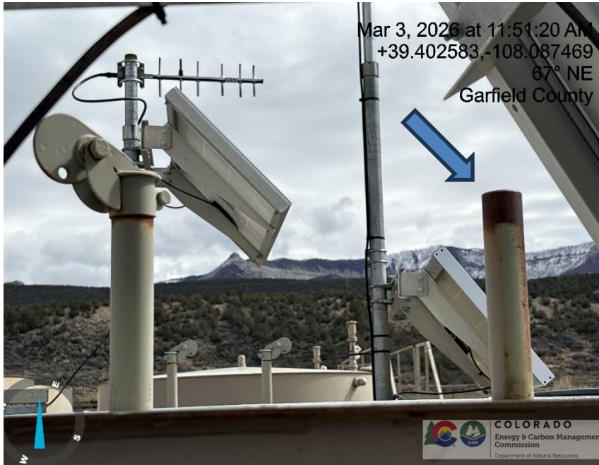
Photo # 4722 From inspection/audit 708908653 conducted on 03/03/2026 - PRV vent line does not comply with CECMC pressure safety device rules
