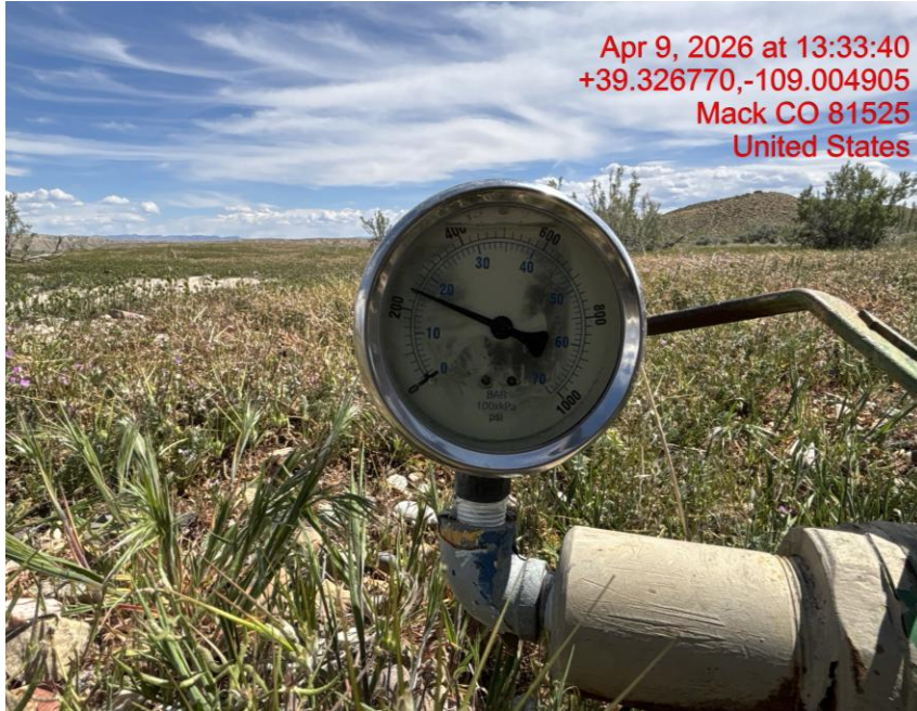
Wellhead Pressure Gauge – Photo #03500
