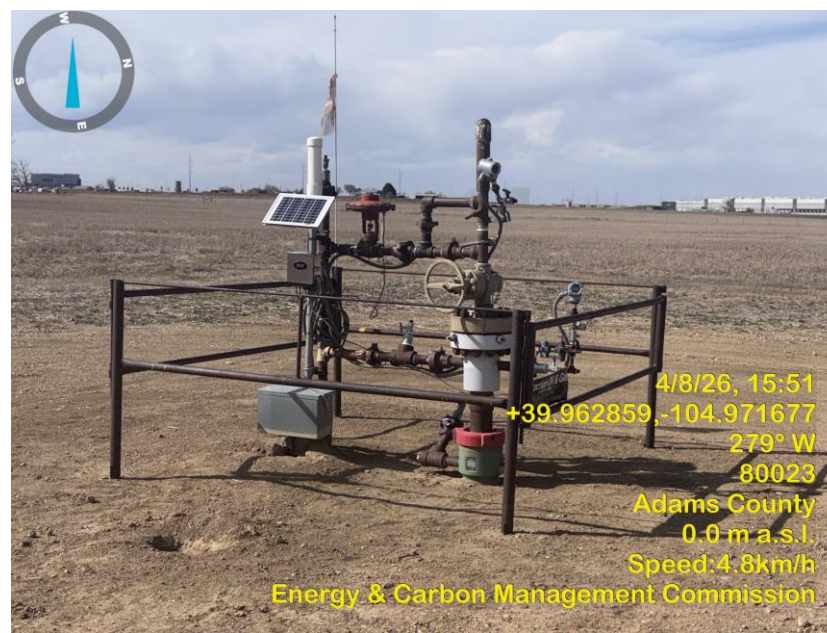
Photo 8 Wellhead.
