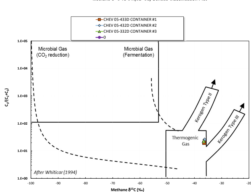
Methane \delta^{13}\text{C} vs C1/(C2+C3) Genetic Classification Plot
