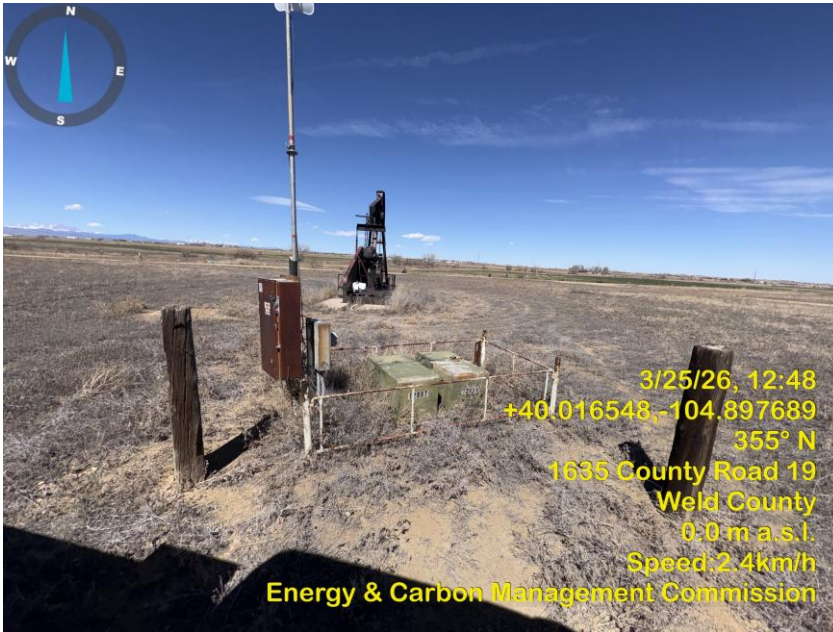
Photo 3 Ancillary equipment.
