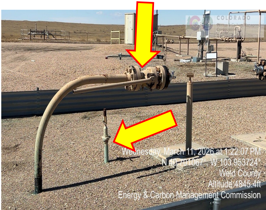
Photo 9 – Unmarked Risers
