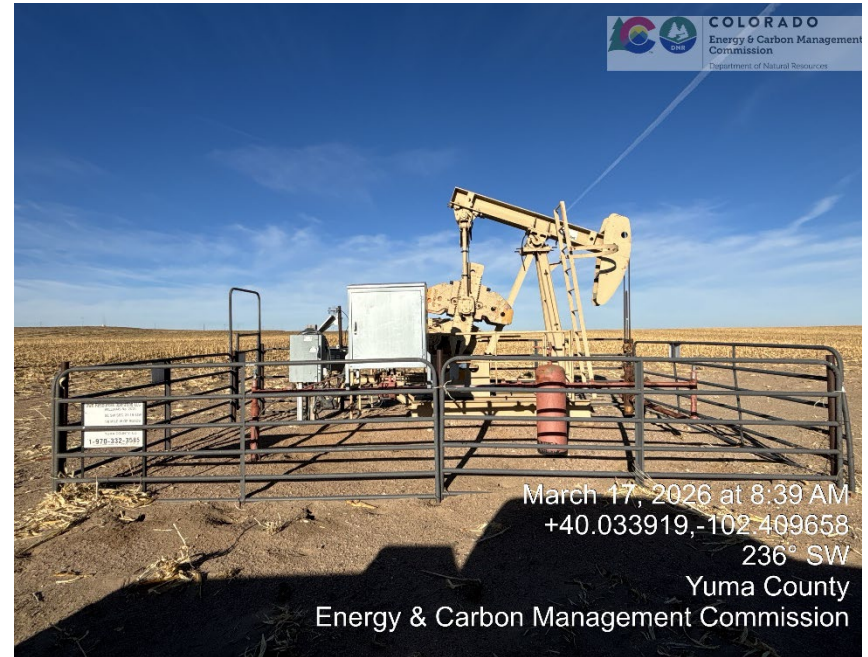
Meter run, PU, and Wellhead
