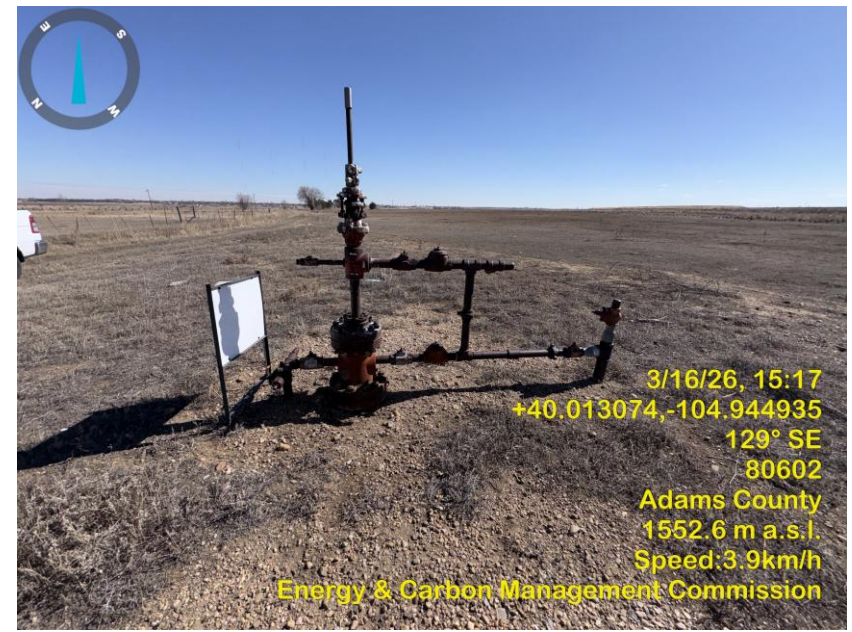
Photo 4 Wellhead.
