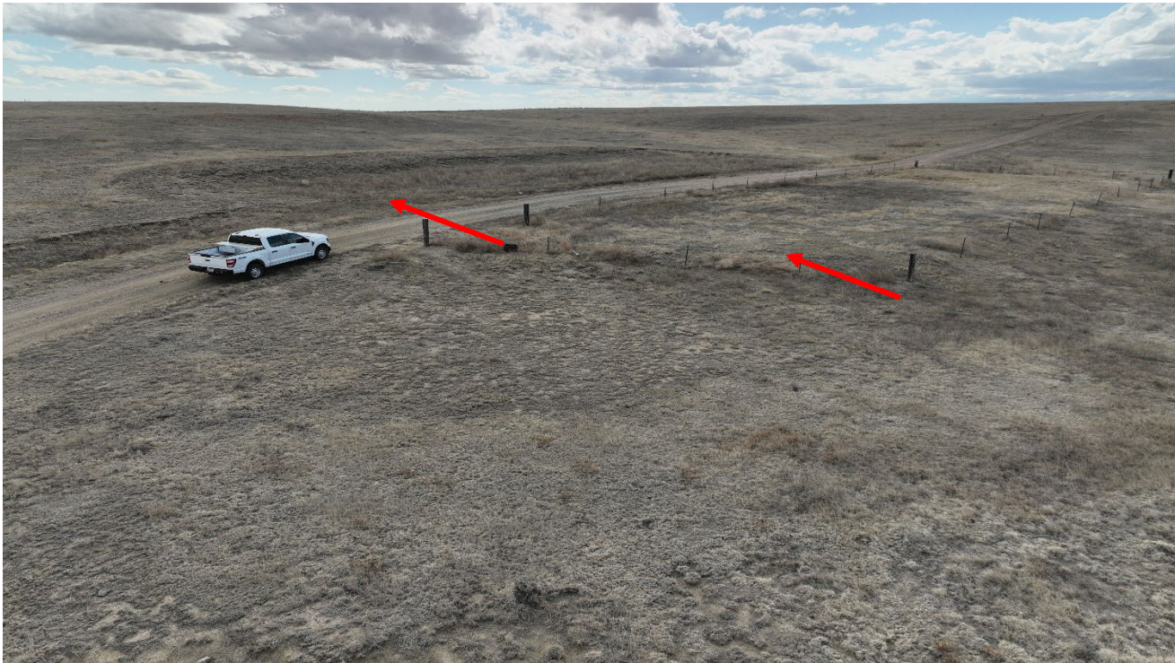
Photo 2. Facing southwest at the location. The fill material needs to be pushed back into the cut slope.
