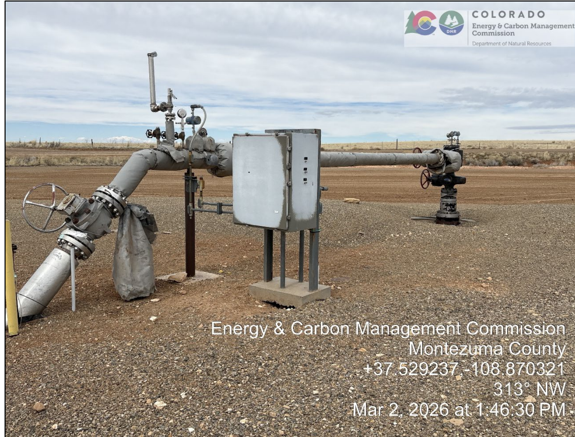
3. Flowline and valves, electrical controls, insulated flow line, wellhead.
