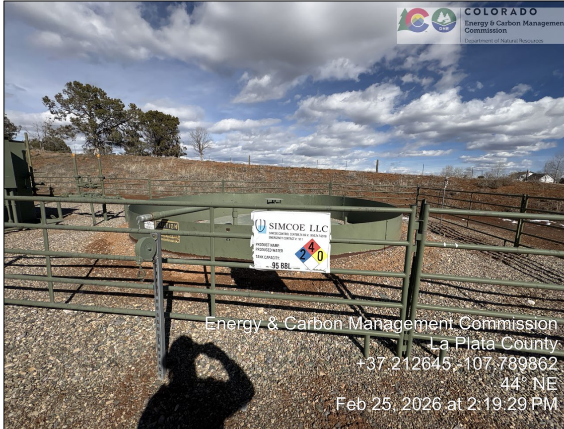
04. Hester 4 produced water tank and secondary containment.
