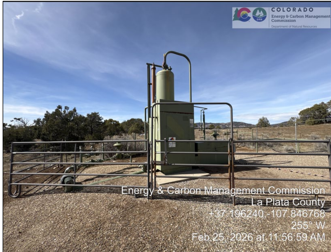
04. Vertical heated separator. Bird protector on stack.
