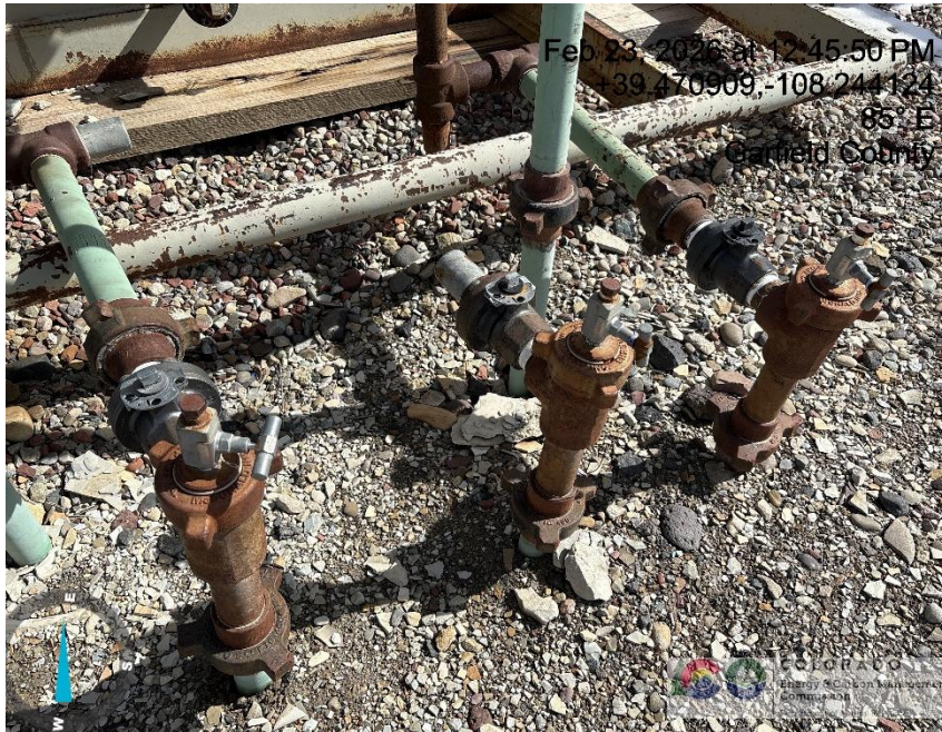
Photo # 2341 Unused flowline lacks lockout tagout (OOSLAT)
