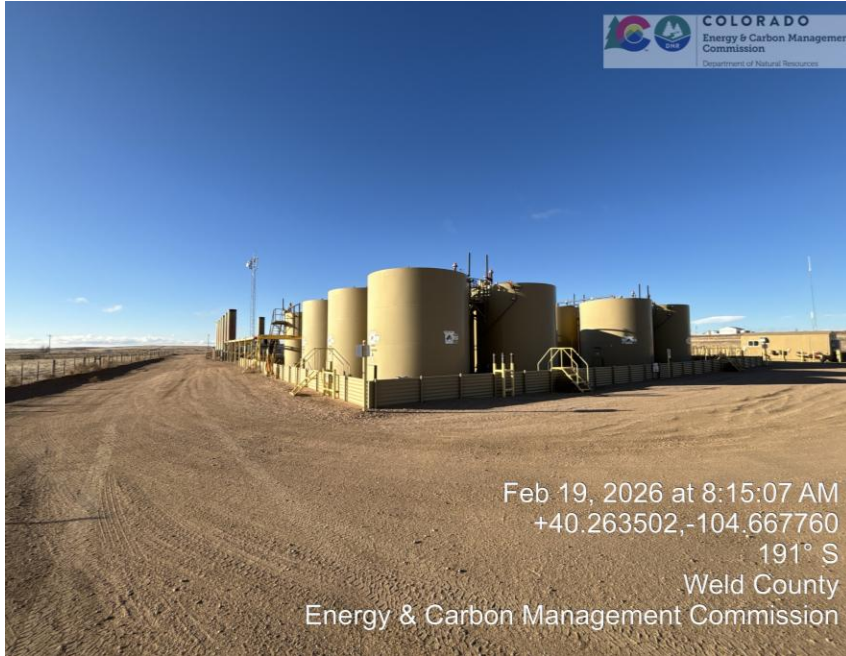
Photo 5 tank battery and equipment
