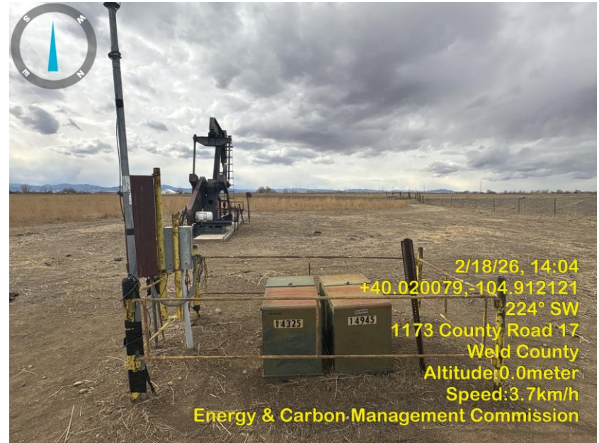
Photo 6 Electric panel, meter box & transformers.
