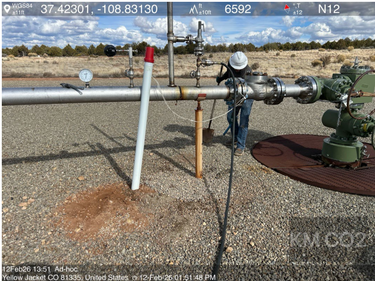
Photo #3. View of the GP-25 flowline and relief valve piping, with impacted soils removed.
