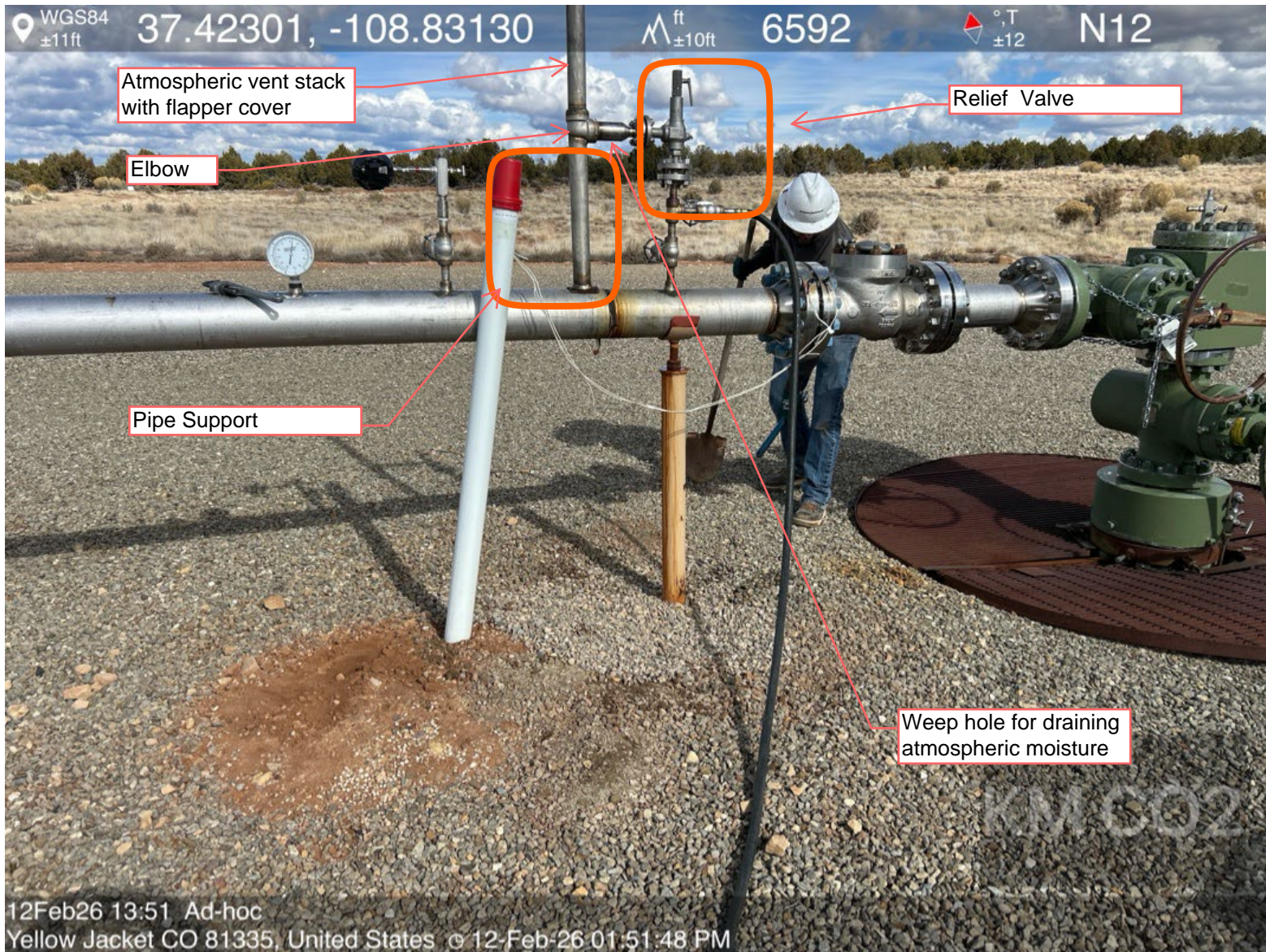
Figure #1. Labeling of the components of the GP-25 flowline assembly.
