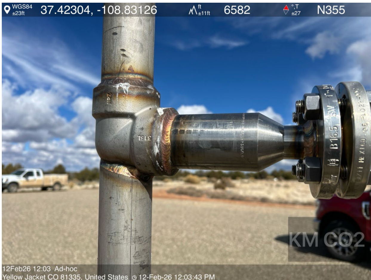
Photo #2. Close up view of the GP-25 flowline relief valve piping, where water was observed leaking. The drip leak on the relief valve piping was terminated.
