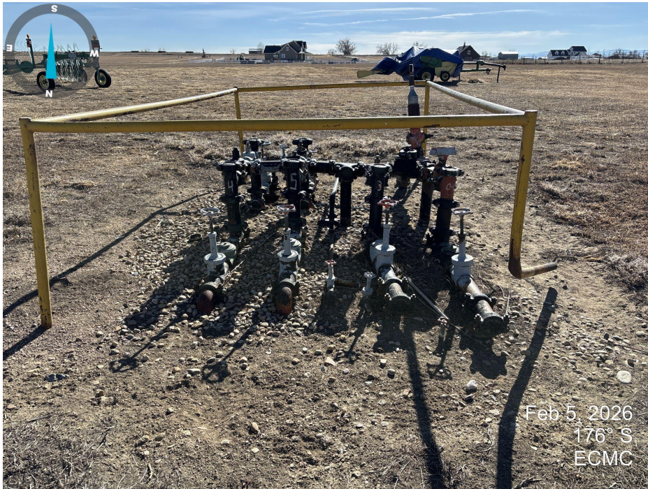
Photo 1. Looking south at the flowline riser station. The equipment is located approximately 250ft northwest of well API 123-07779.
