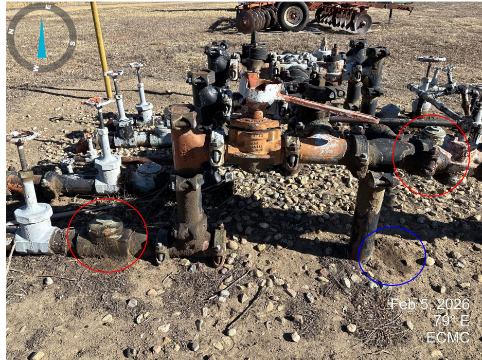
Photo 2. Photo taken looking east at the west side of the equipment. Leaking joints (red circle) and stained soil (blue circles) are present on the equipment.
