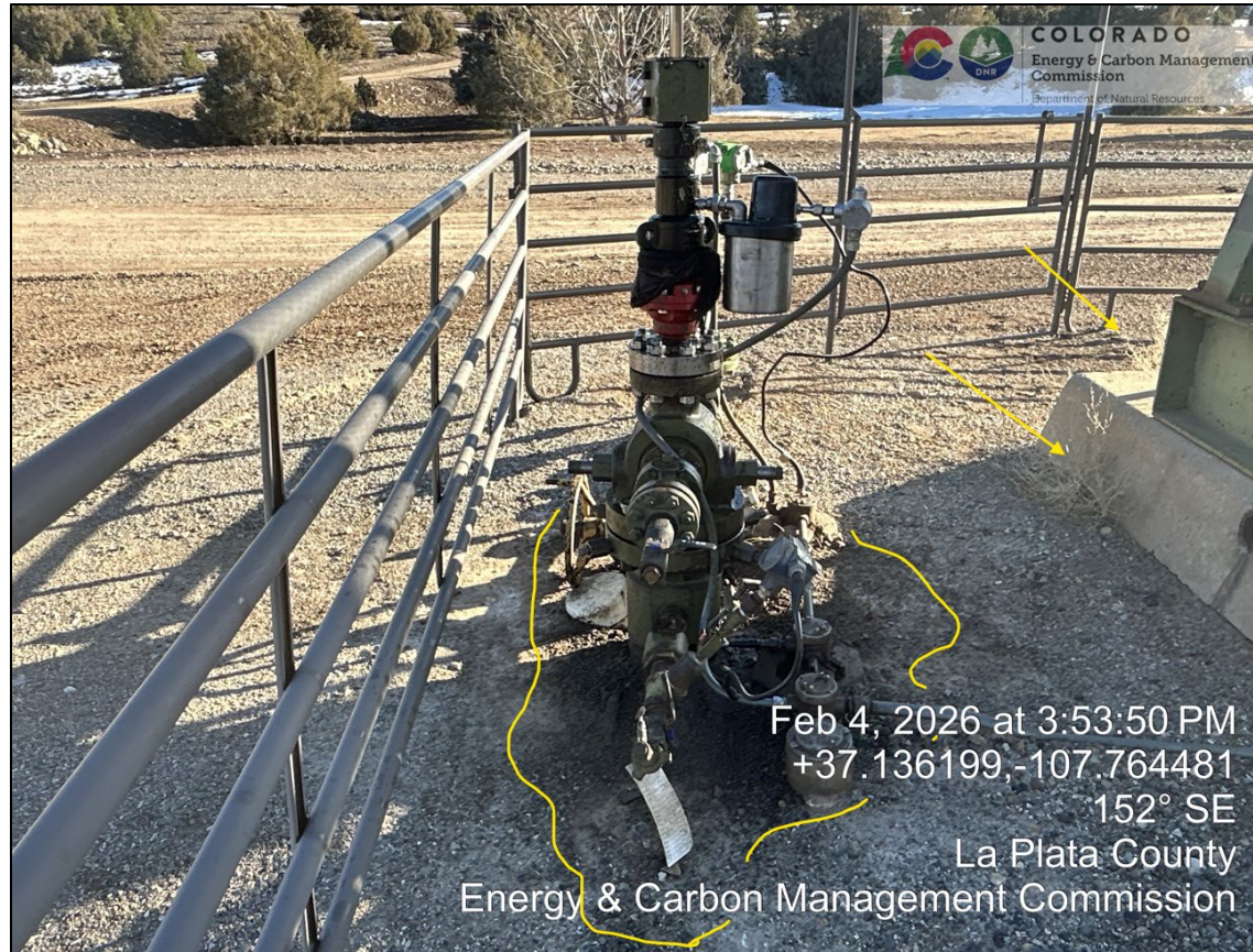
7. Wellhead. Note oil stain on ground (outlined in yellow) and dead vegetative debris (arrow). View looking south.
