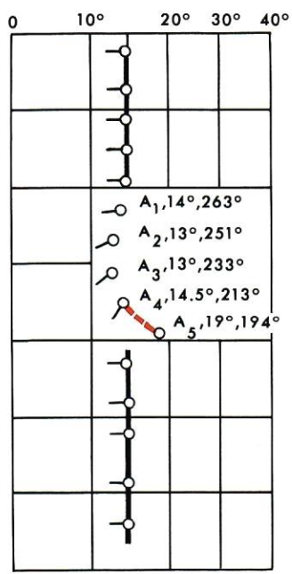
Fig. 10. Arrow Plot
