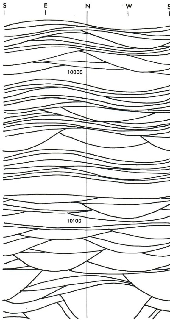
Fig. 6. FAST Plot
