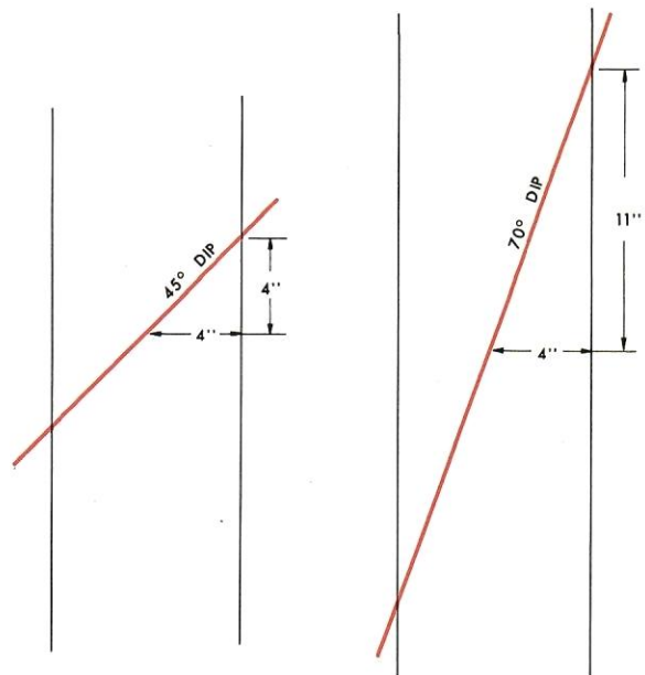
Fig. 3. Search Angle
