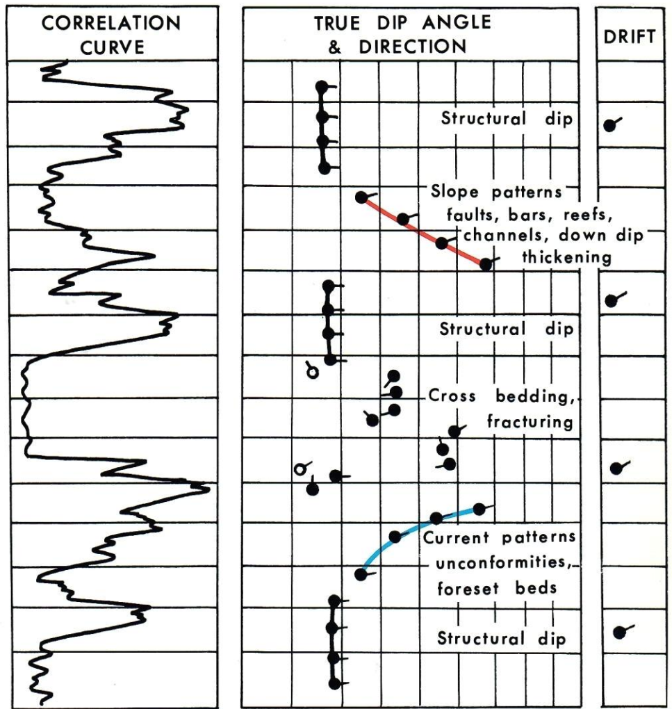
Fig. 4. Arrow Plot
