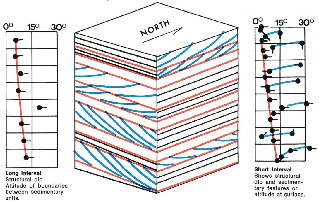
Fig. 1. Correlation Length
