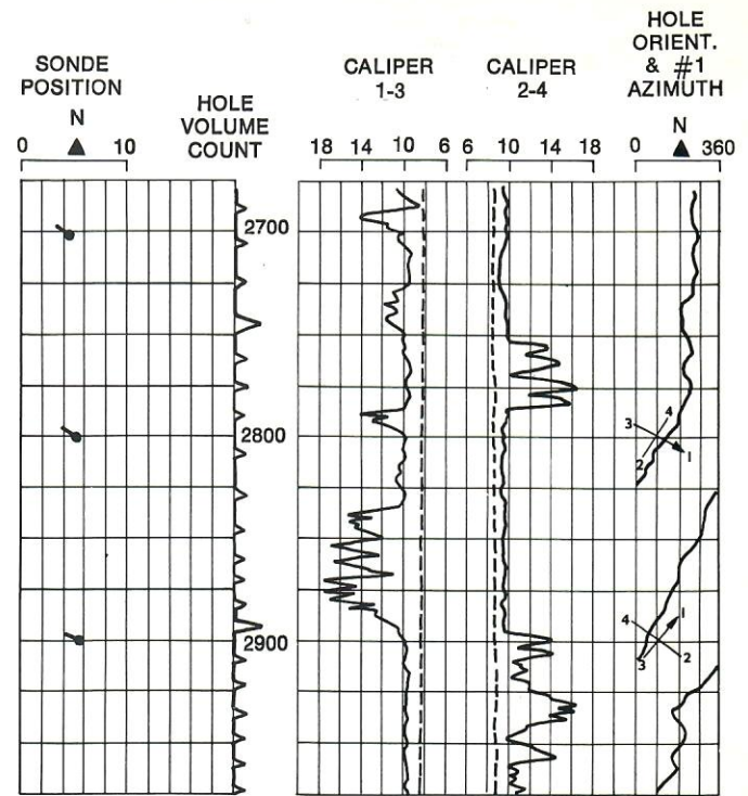
Fig. 12. Borehole Geometry
