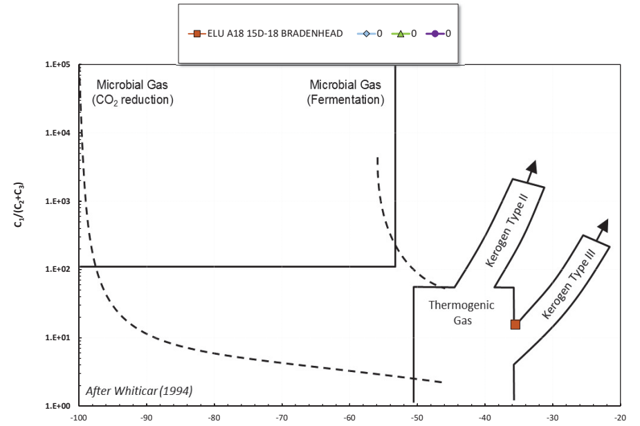
Methane \delta^{13}\text{C} vs \text{C}_1/(\text{C}_2+\text{C}_3) Genetic Classification Plot
