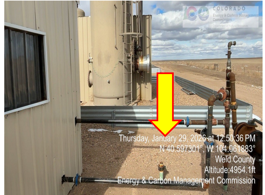
Photo 24 – Unmarked Riser
