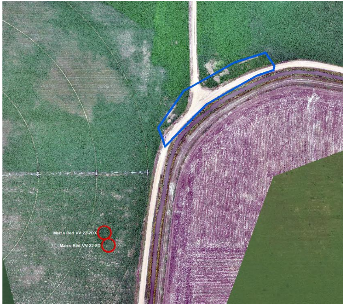
Photo 2. Orthomosaic (drone) imagery taken 10/7/2025 and NAIP imagery (2023) illustrating the well locations (red circles) and associated tank battery (blue polygon).
