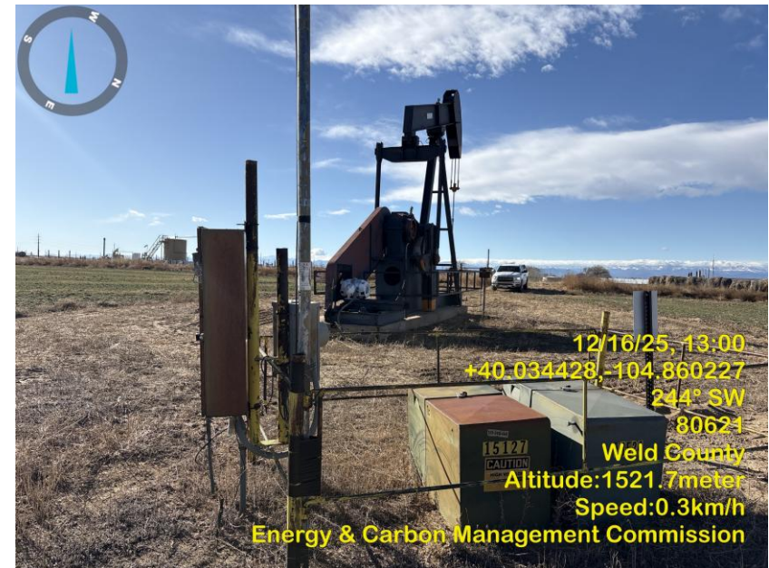
Photo 4 Ancillary equipment.
