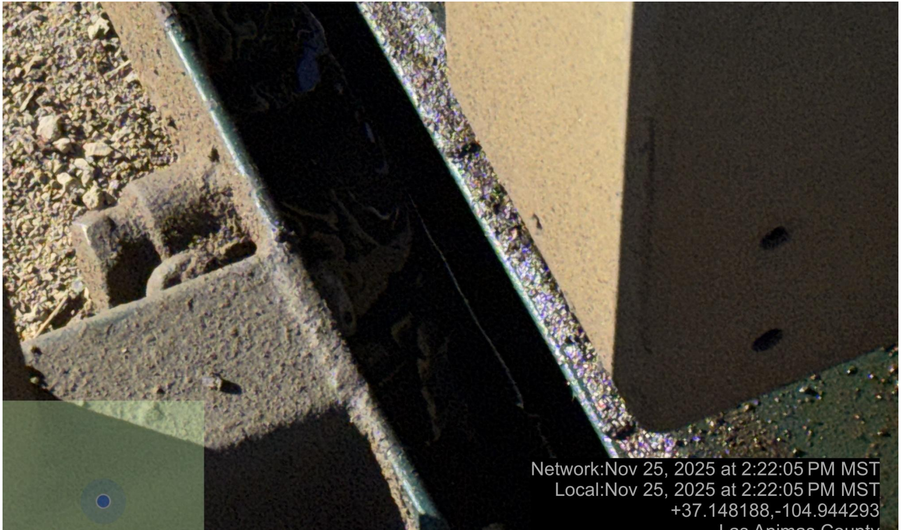
PHOTO 6: OILY WASTE IN COMPRESSOR SKID. DRAIN OILY WASTE REPAIR ALL LEAKS AND REMOVE IMPACTED SOIL PER RULE 1002..(2).D & 1002.f.(2)B, Comply with general provisions of the oil and gas act for wildlife protection AND SB-181. 24 HOURS TO DRAIN OILY WASTE, 10 DAYS TO REPAIR LEAKING EQUIPMENT.
