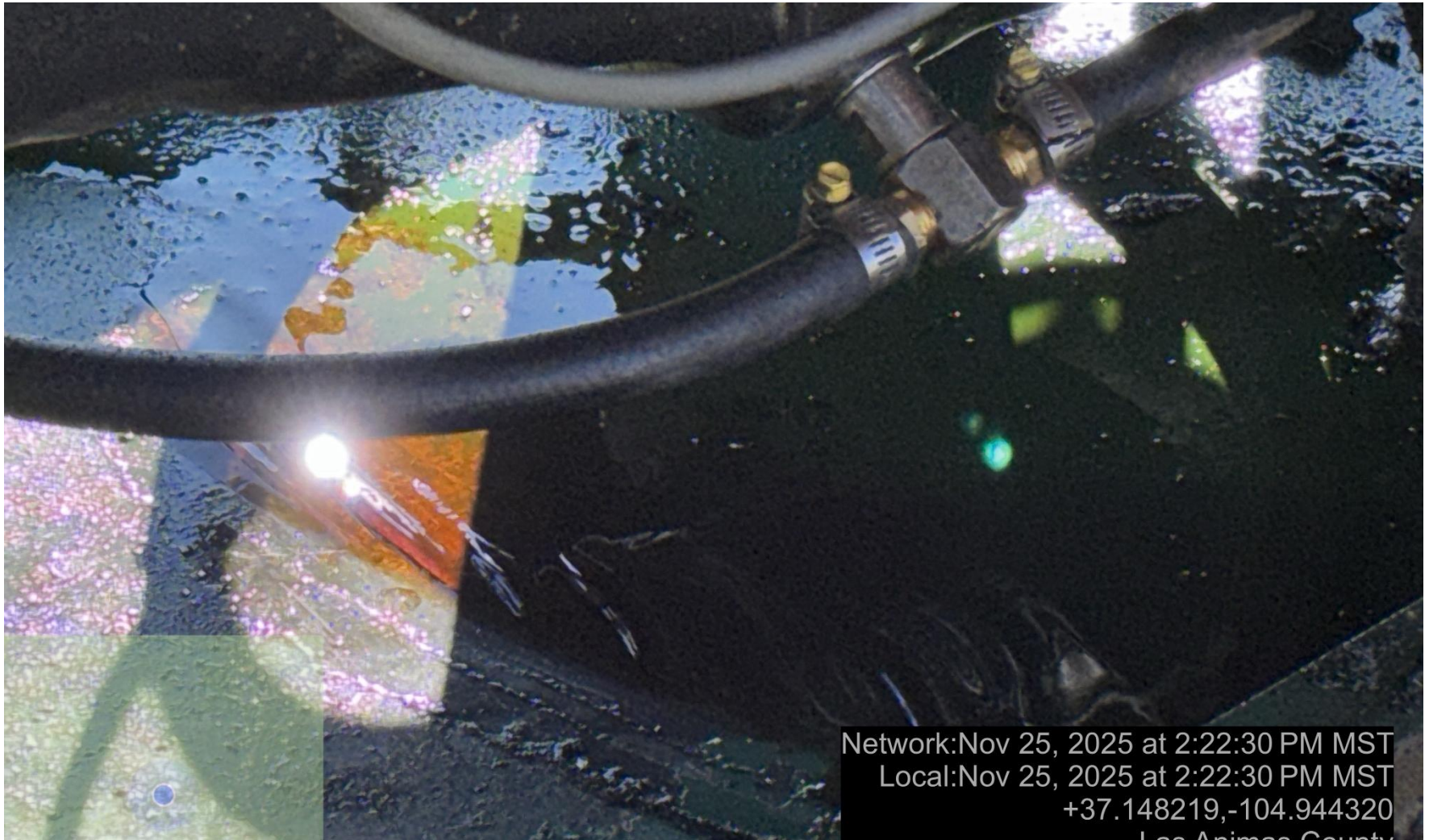
PHOTO 7: OILY WASTE IN COMPRESSOR SKID. DRAIN OILY WASTE REPAIR ALL LEAKS AND REMOVE IMPACTED SOIL PER RULE 1002.(2).D & 1002.f.(2)B, Comply with general provisions of the oil and gas act for wildlife protection AND SB-181. CA DATE 11-26-2025.
