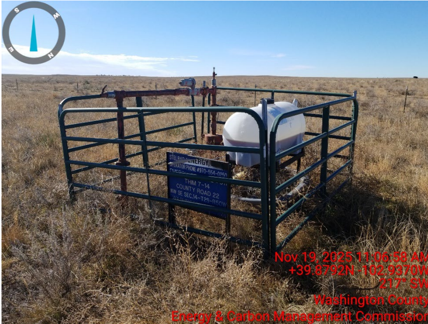
1. Wellhead and chemical tank
