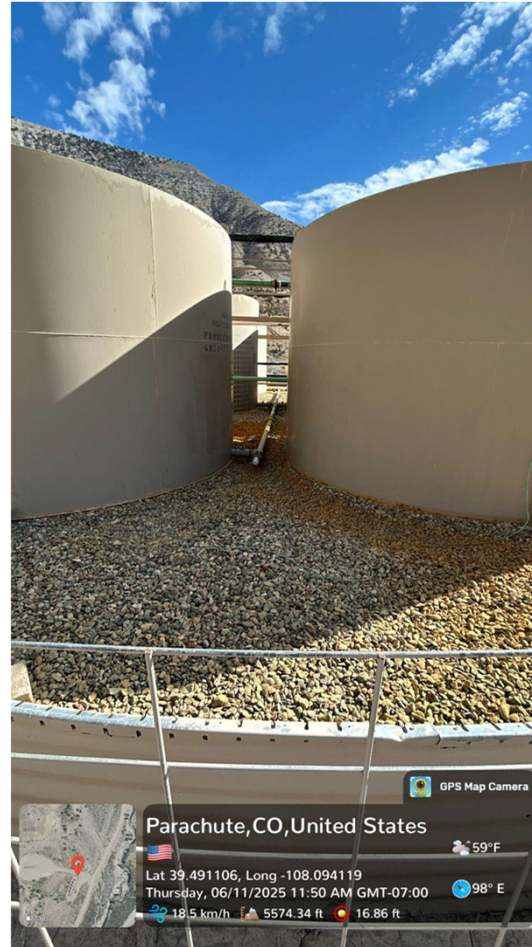
Photo 5– Facing East viewing hydrovaced spill area
