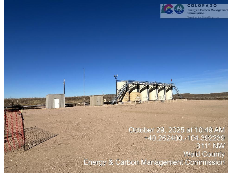
Production Tanks
