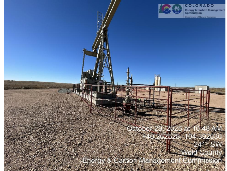
Unused pumping unit- no prime mover
