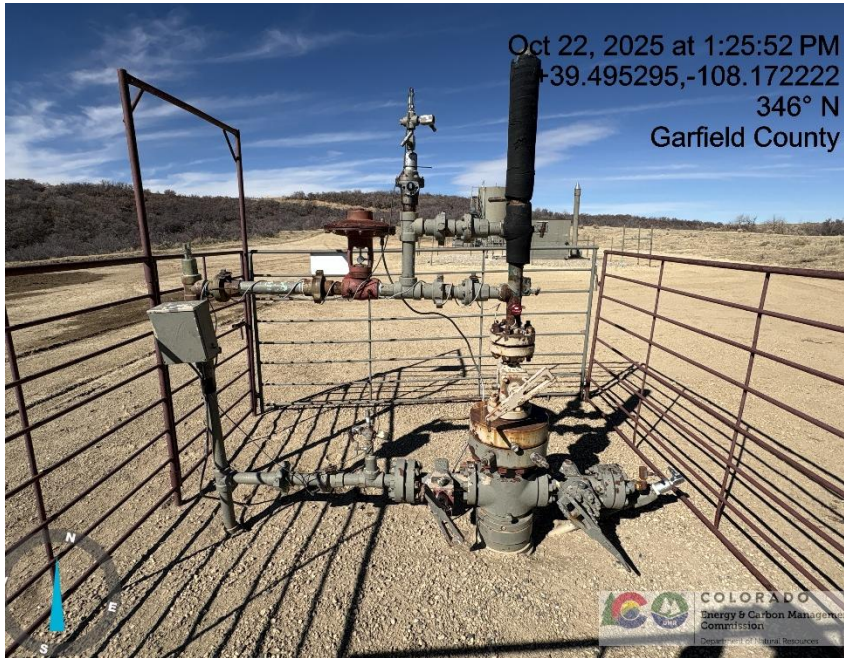
Photo # 1493 PUCKETT 234-25 wellhead (parasite line plumbed to surface & SC BH buried/not in compliance with CECMC Rule 419)
