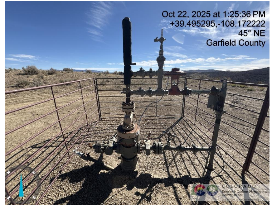
Photo # 1492 PUCKETT 234-25 wellhead (parasite line plumbed to surface & SC BH buried/not in compliance with CECMC Rule 419)
