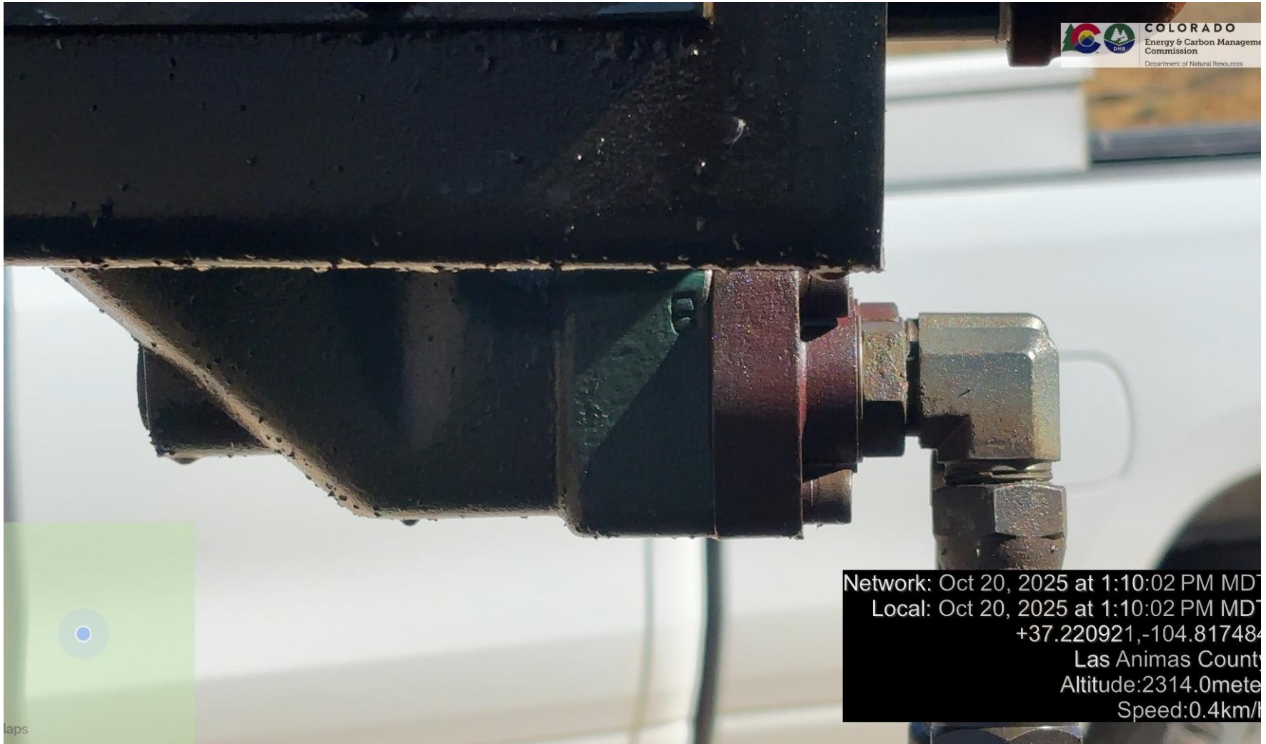
PHOTO 4: DRIVEHEAD IS LEAKING HYDRAULIC OIL. Securely fasten all valves, pipes, fittings, and Production Facilities to ensure good mechanical condition, inspect at regular intervals and maintain in good mechanical condition per Rule 608.e. CA DATE 10-21-2025.
