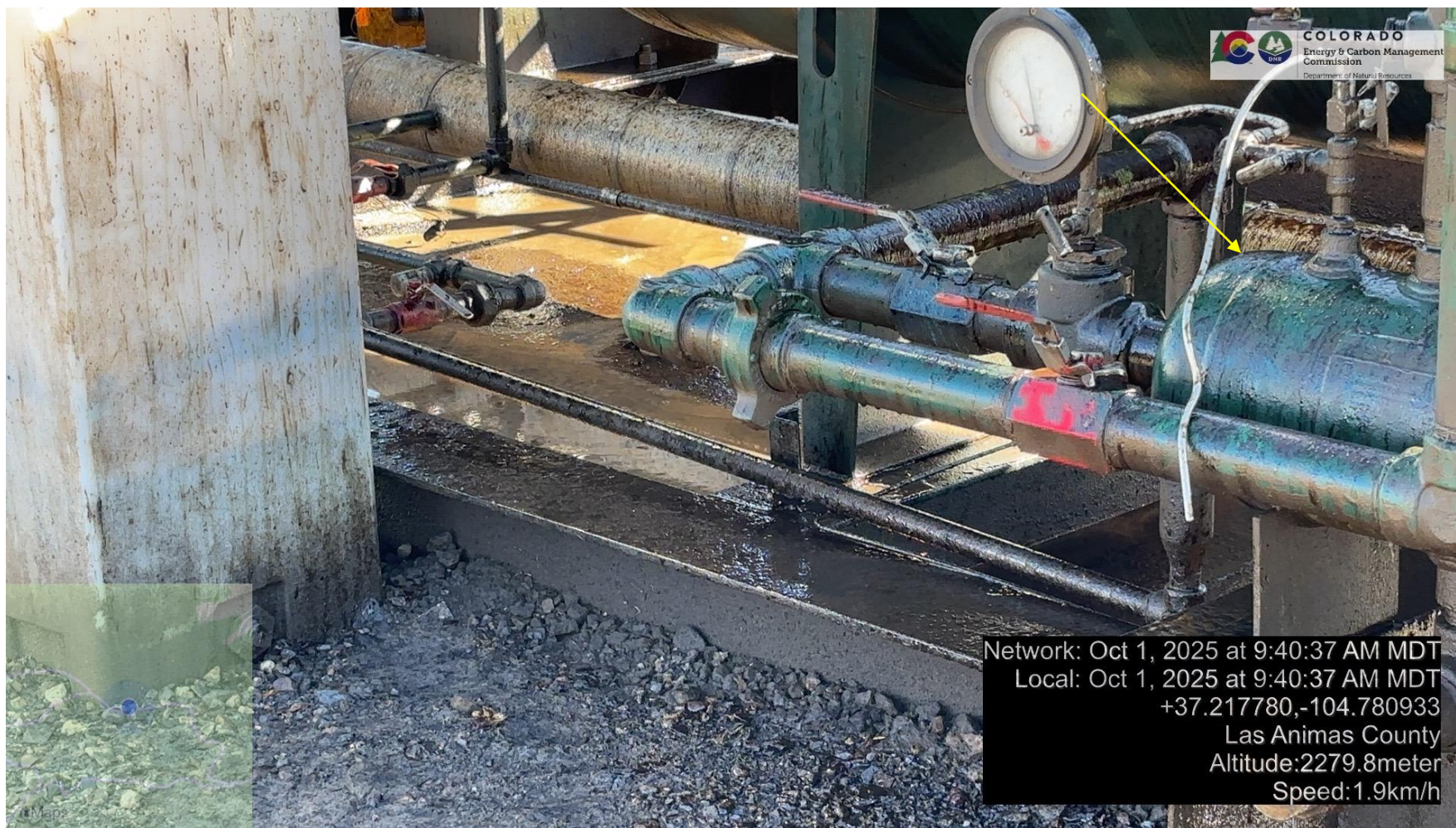
PHOTO 7: CLOSER IMAGE OF THE EQUIPMENT WITH THE MECHANICAL FAILURE. OPERATOR INFORMED ECMC STAFF THAT THE FILTER MARKED BY THE ARROW PLUGGED AND CAUSED THE FAILURE.
