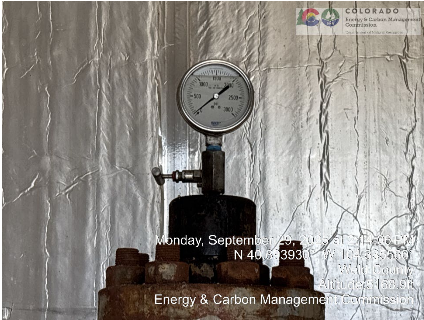
Photo 3 – Tubing Gauge
