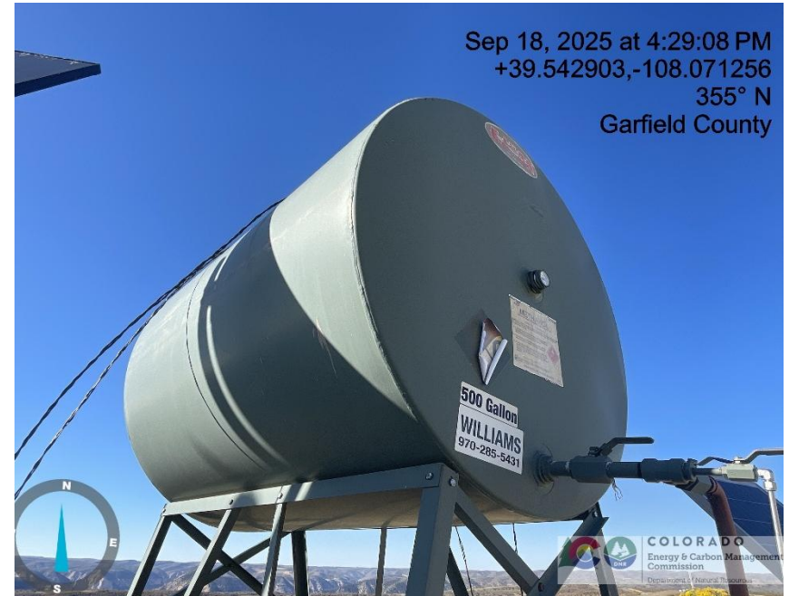
Photo # 1212 Labeling on methanol tank weathered & damaged/starting to become illegible
