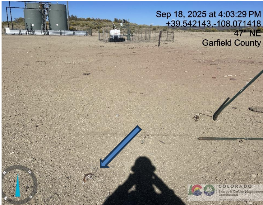
Photo # 1205 Unmarked deadman
