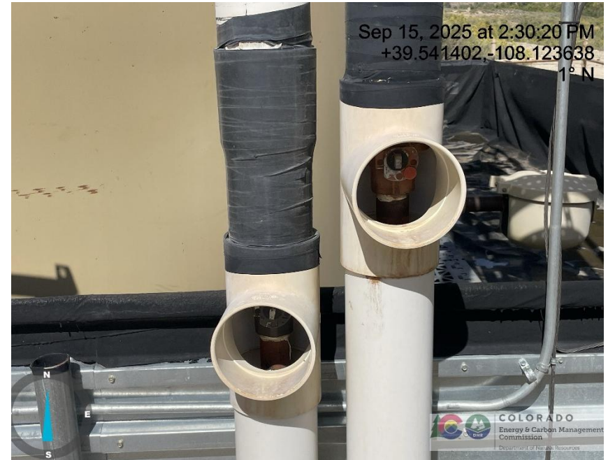
Photo # 9376 Flowline heating insulation open ended /wildlife hazard/available for entry by wildlife
