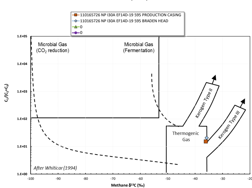
Methane \delta^{13}\text{C} vs \text{C}_1/(\text{C}_2+\text{C}_3) Genetic Classification Plot
