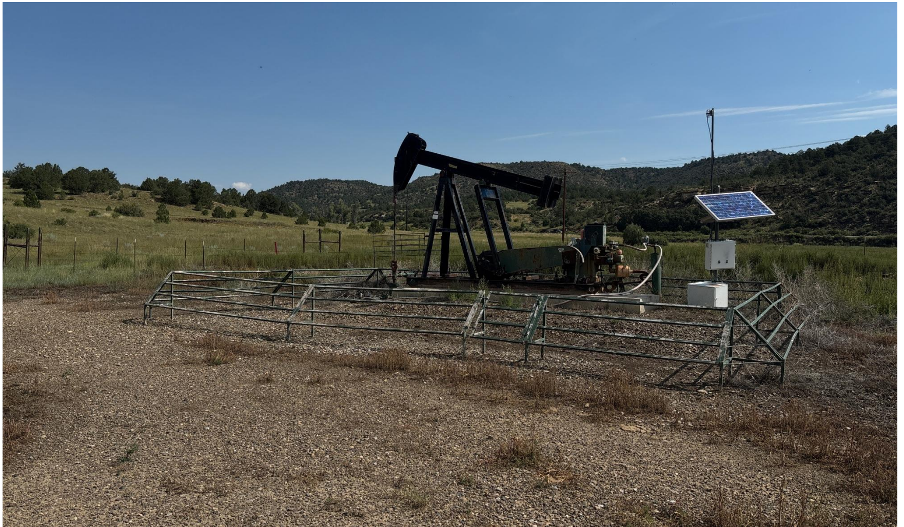
PHOTO 2: WELLHEAD AND EQUIPMENT.
