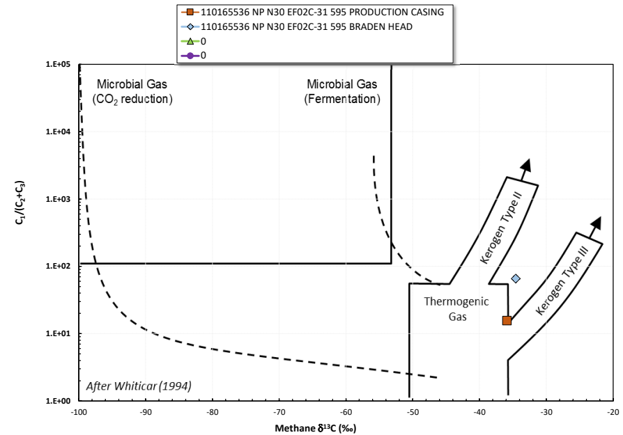
Methane \delta^{13}\text{C} vs \text{C}_1/(\text{C}_2+\text{C}_3) Genetic Classification Plot
