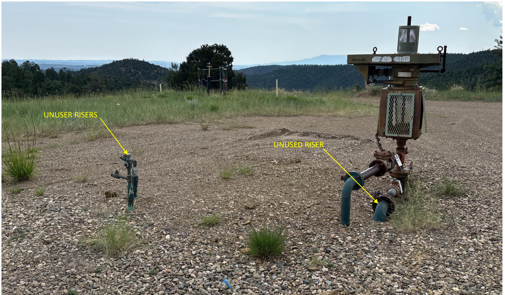
PHOTO 3: WELLHEAD AND EQUIPMENT/ UNUSED EQUIPMENT (ONE 3" RISER NEXT TO WELLHEAD AND TWO 2" RISERS NORTH OF WELLHEAD) NOT IN USE OR MARKED. MARK OR REMOVE UNUSED EQUIPMENT PER RULE 606.
