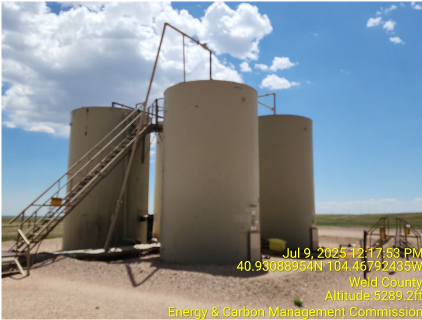
Photo 7 – Tank Battery
