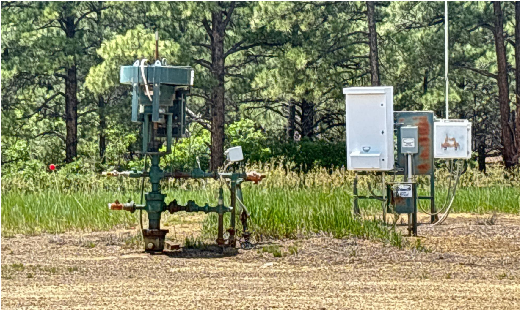
PHOTO 4: WELLHEAD AND EQUIPMENT, WEEDS NEED MAINTAINED AROUND BOTH WELLHEADS.
