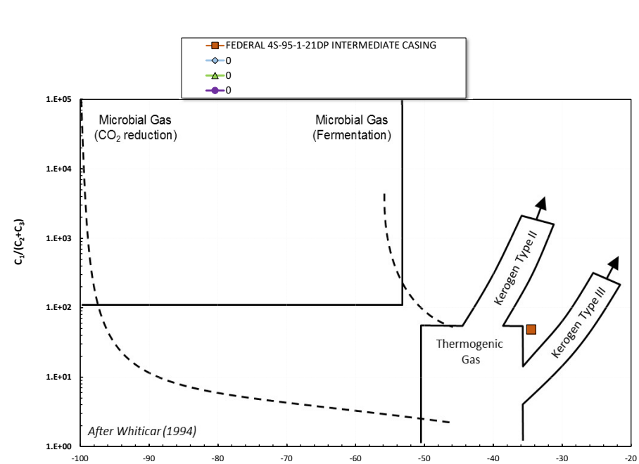
Methane \delta^{13}\text{C} vs C1/(C2+C3) Genetic Classification Plot
