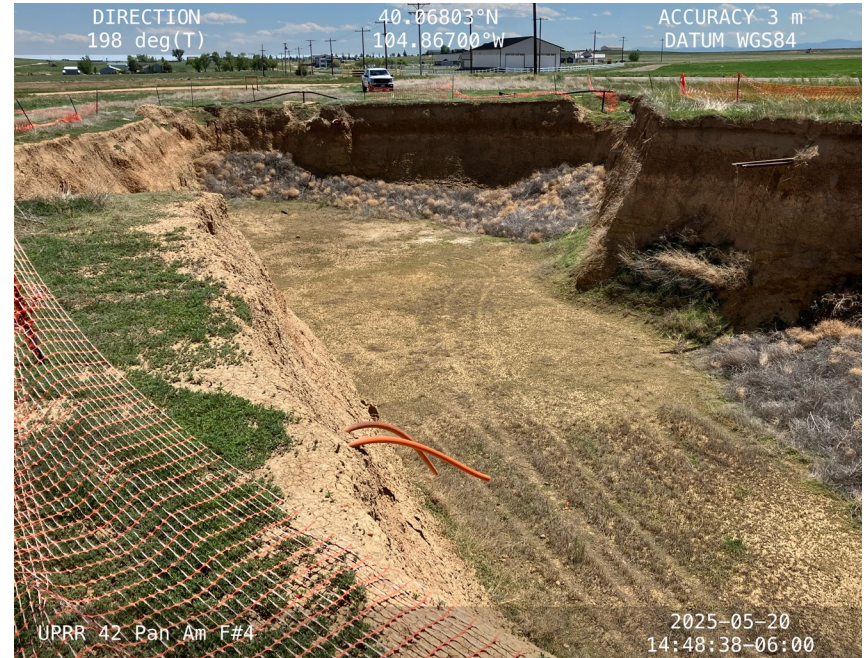
Multiple flowlines of unknown status were observed exposed within the open excavation.
