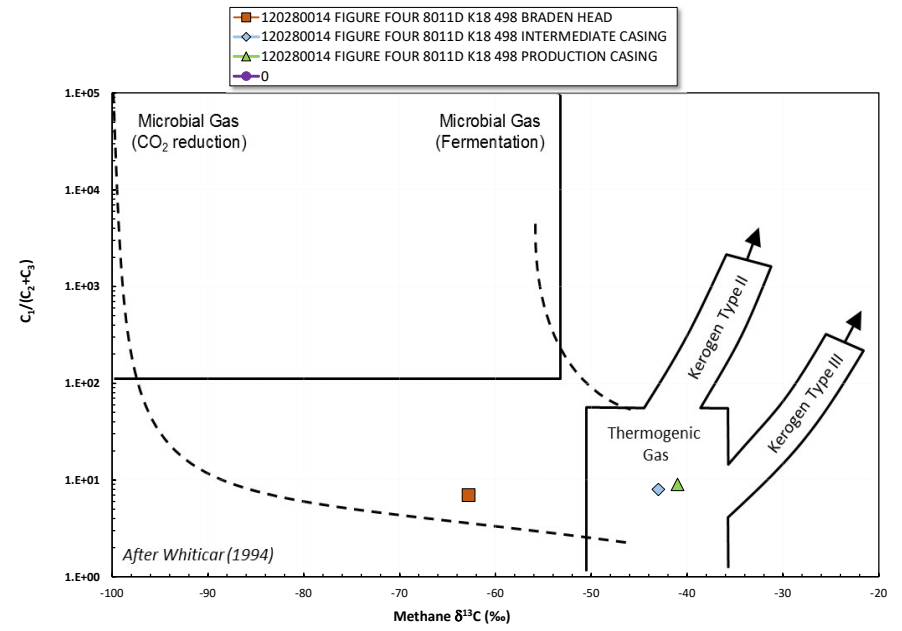
Methane \delta^{13}\text{C} vs C1/(C2+C3) Genetic Classification Plot
