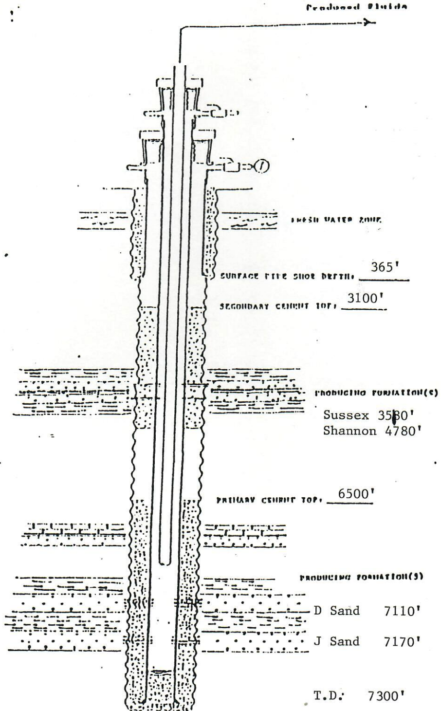
WELLBORE DIAGRAM
